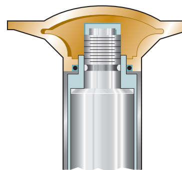
Metal-to-Metal Sleeve Design
